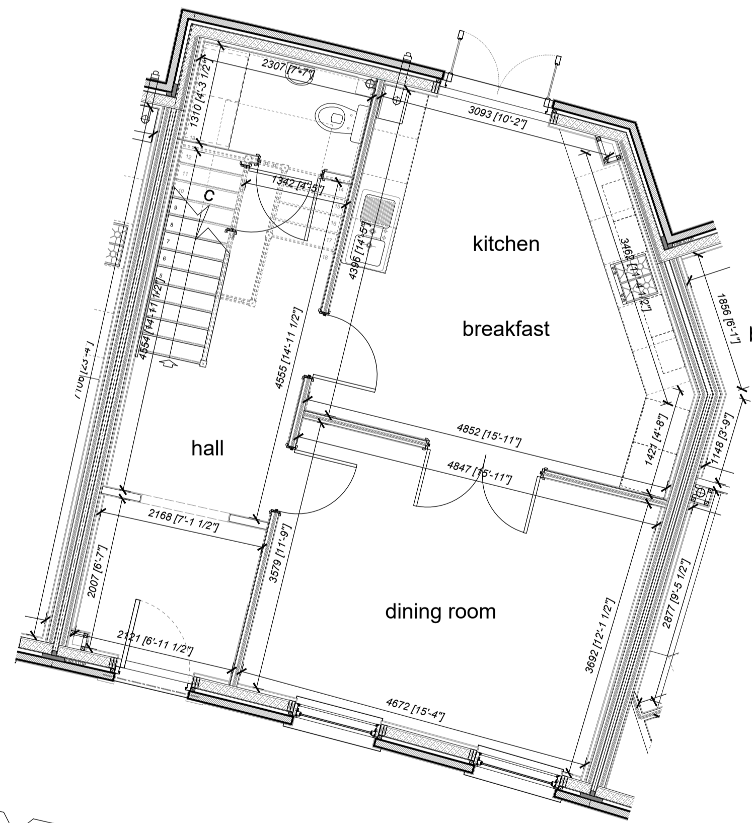
House 13 Ground Floor
