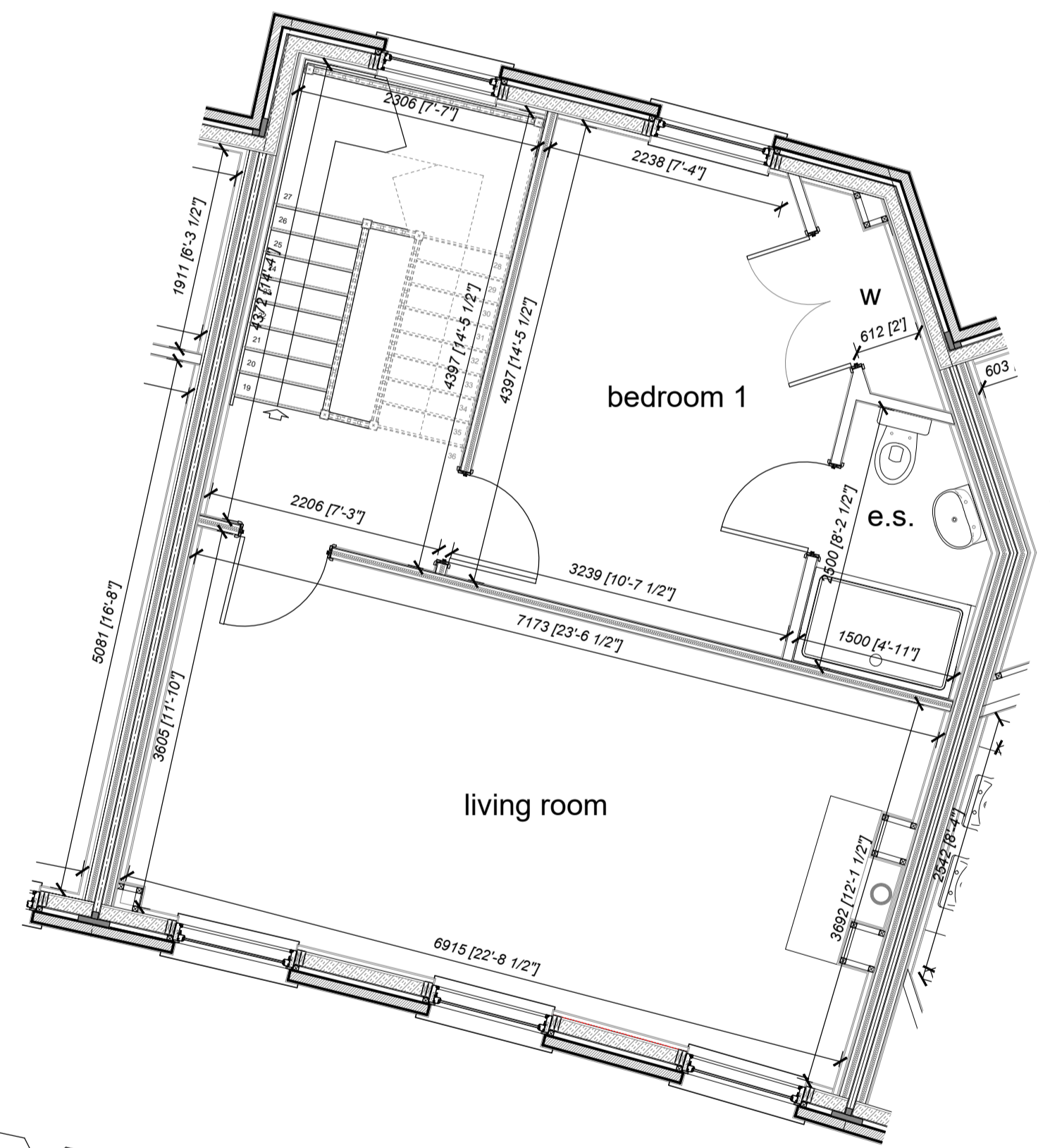
House 13 First Floor
