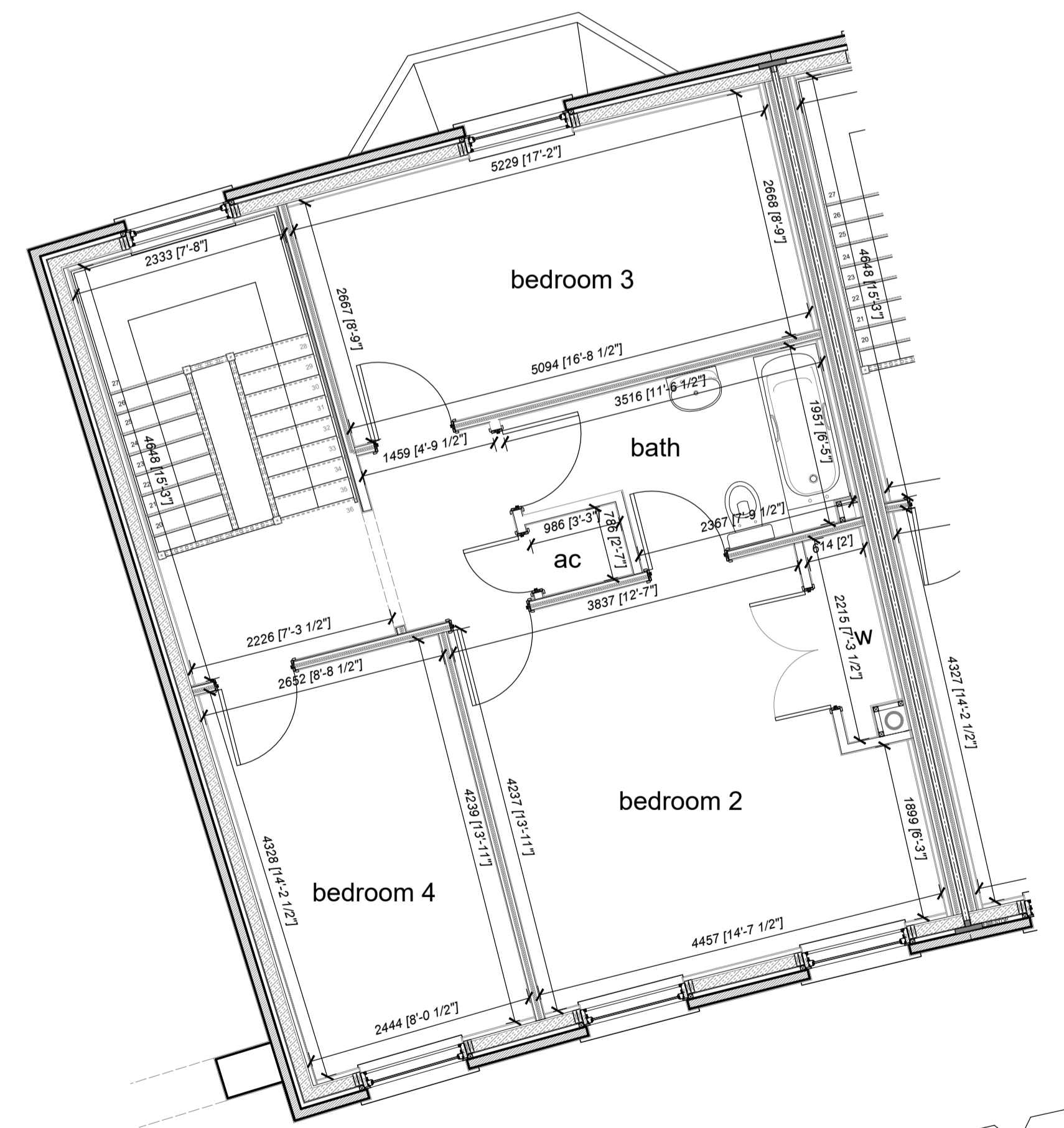
House 07 Second Floor
