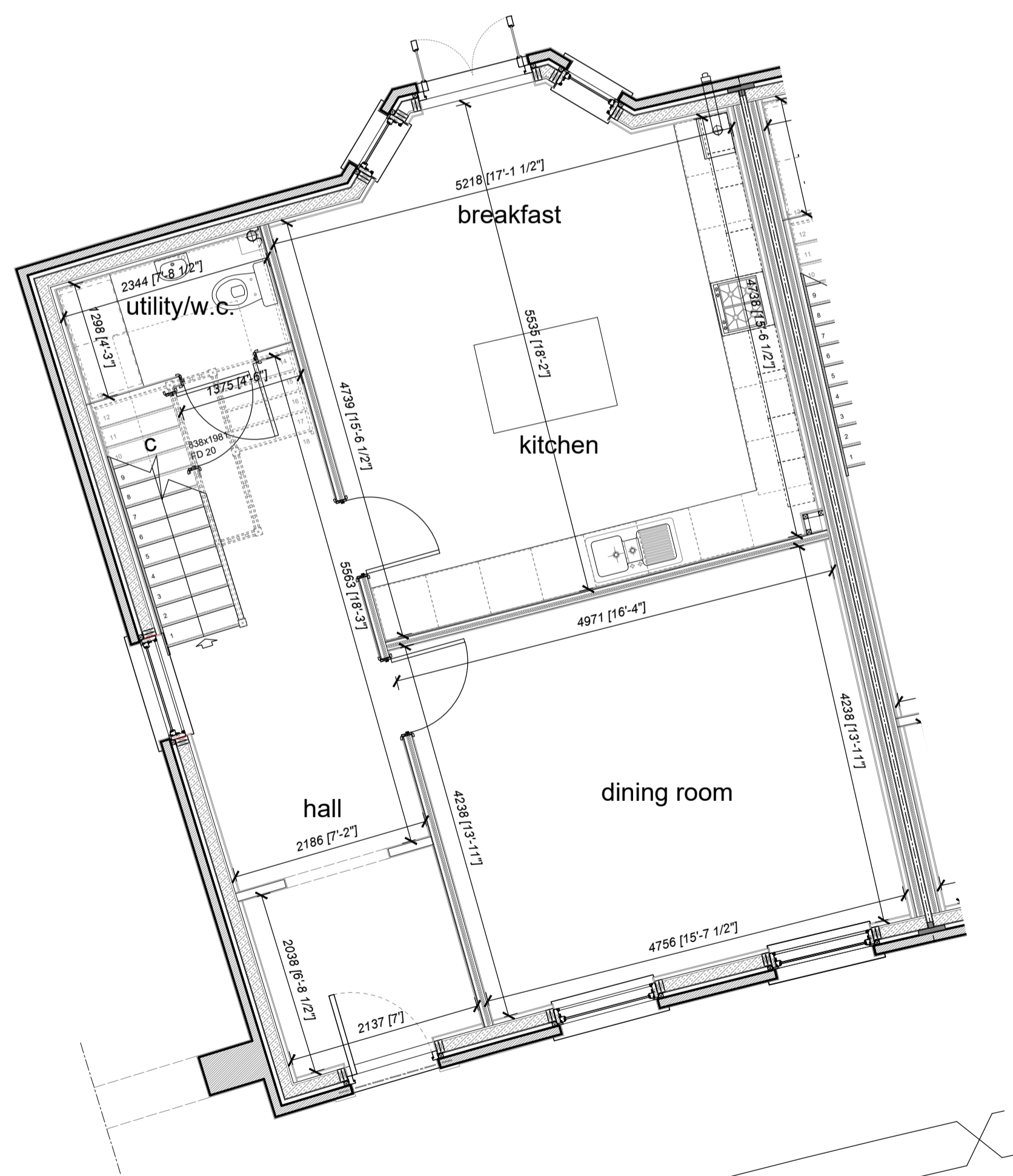
House 07 Ground Floor
